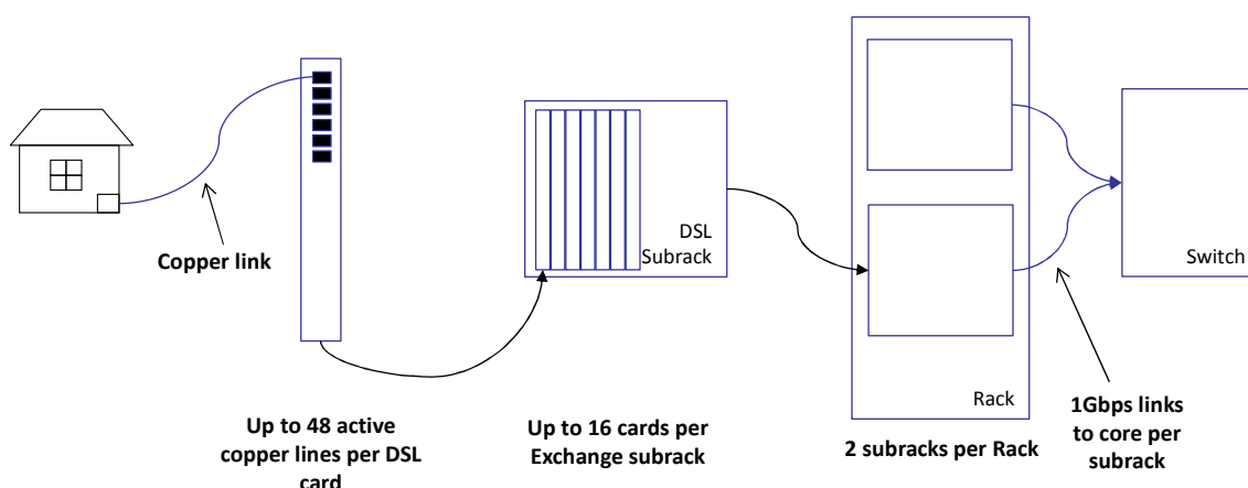
Figure 36 – DSLAMs dimensioning
