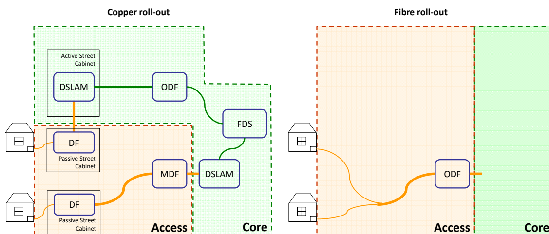
Figure 40 – Demarcation point of the copper and of the fibre networks
