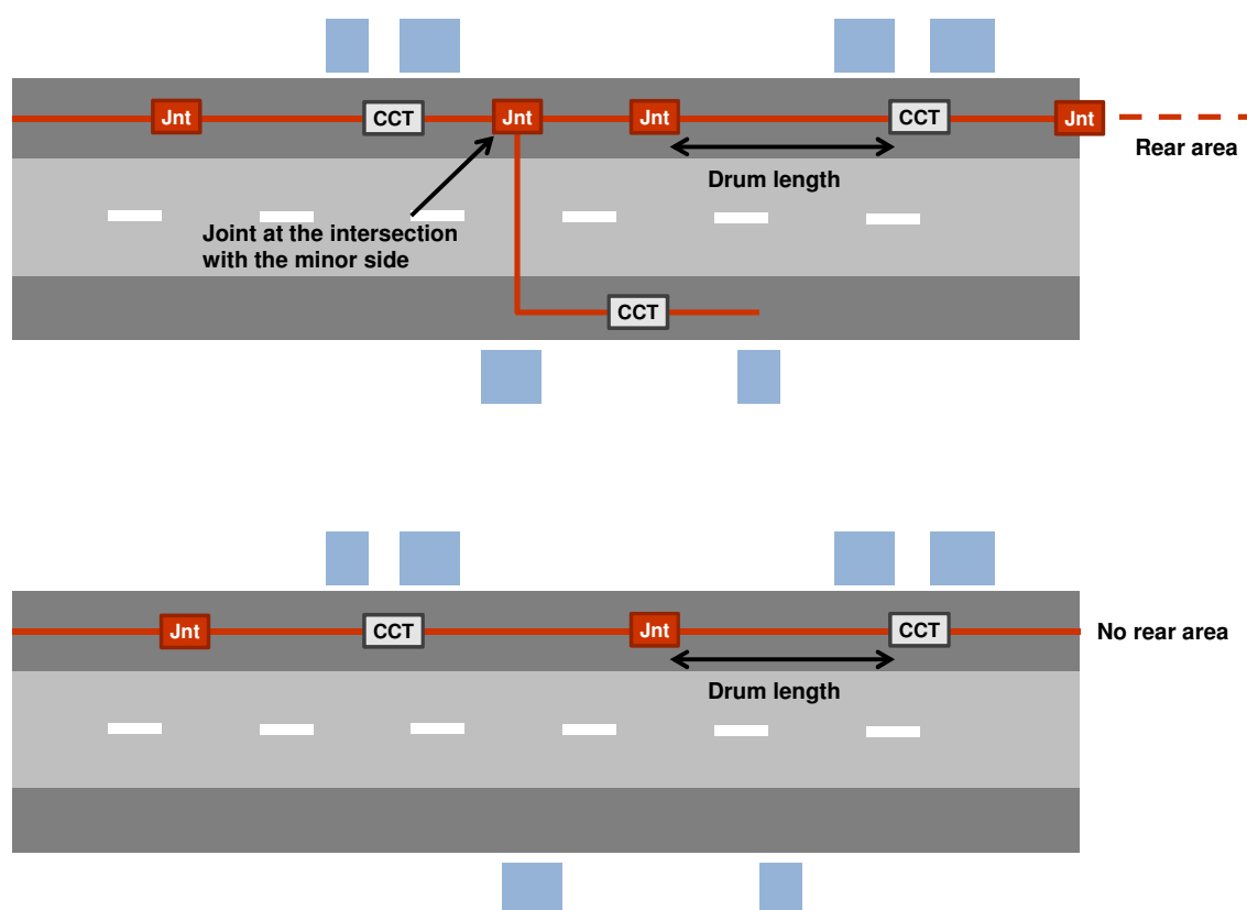
Figure 27 – Joints on the major and minor sides
