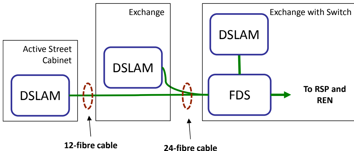
Figure 38 – DSLAM-FDS fibre cables
