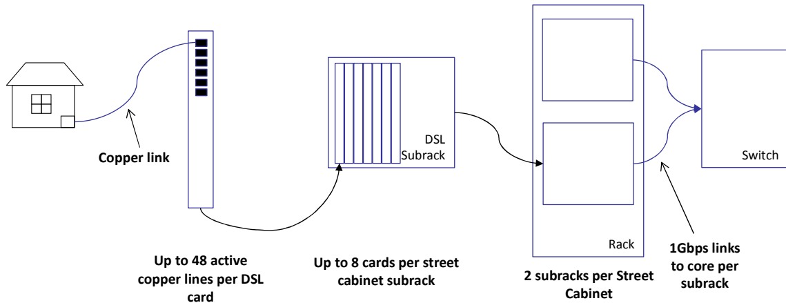
Figure 35 – DSLAMs dimensioning
