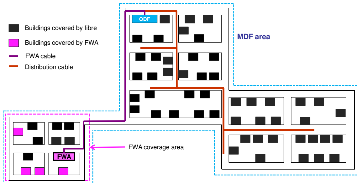
Figure 31 – Architecture of the FWA network
