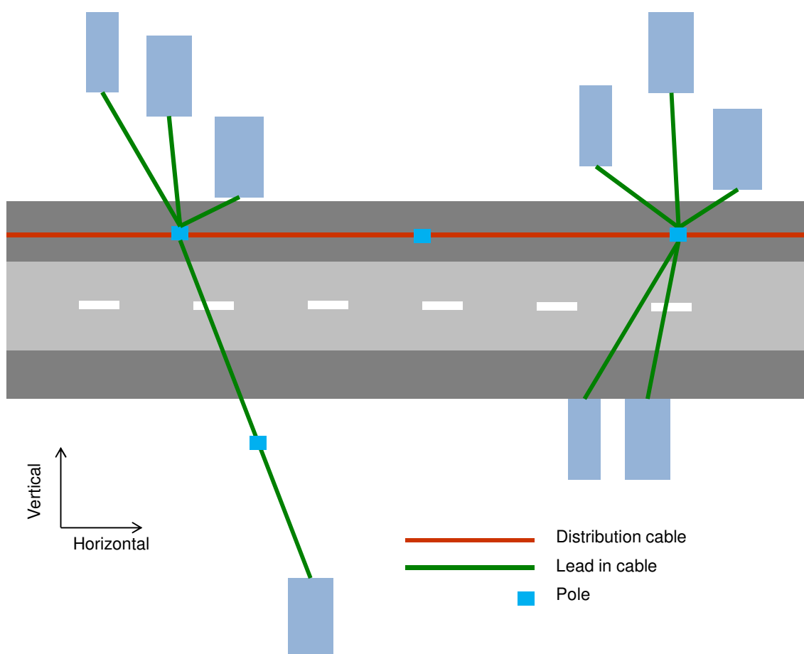
Figure 28 – Location of poles
