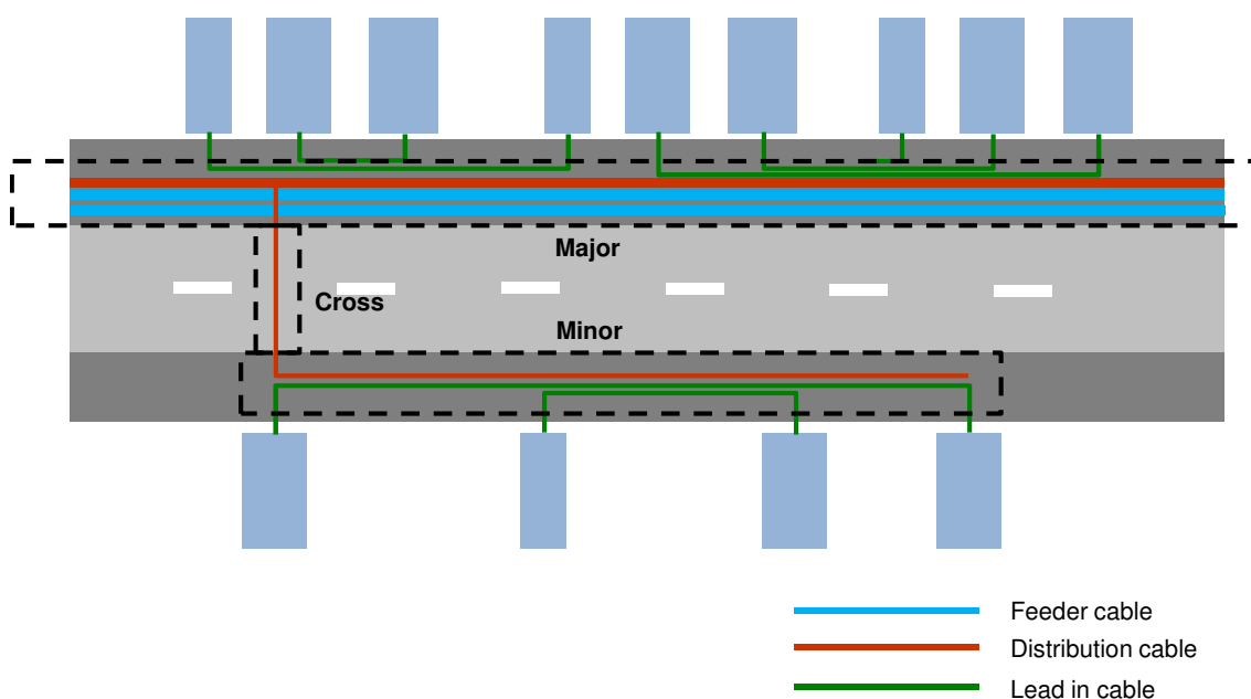
Figure 29 – Horizontal trenches
