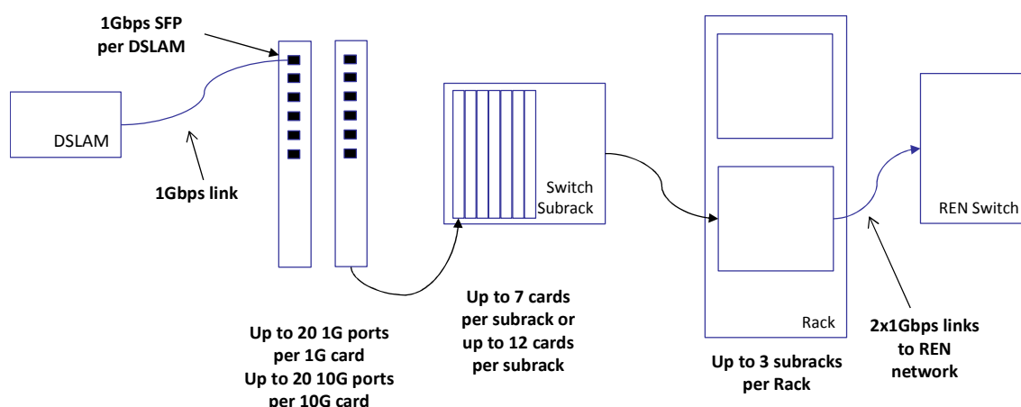
Figure 37 – FDS dimensioning
