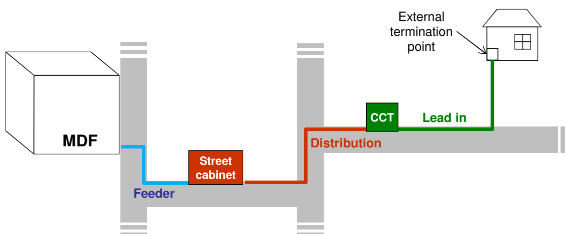
Figure 22 – Architecture of the local access copper network
