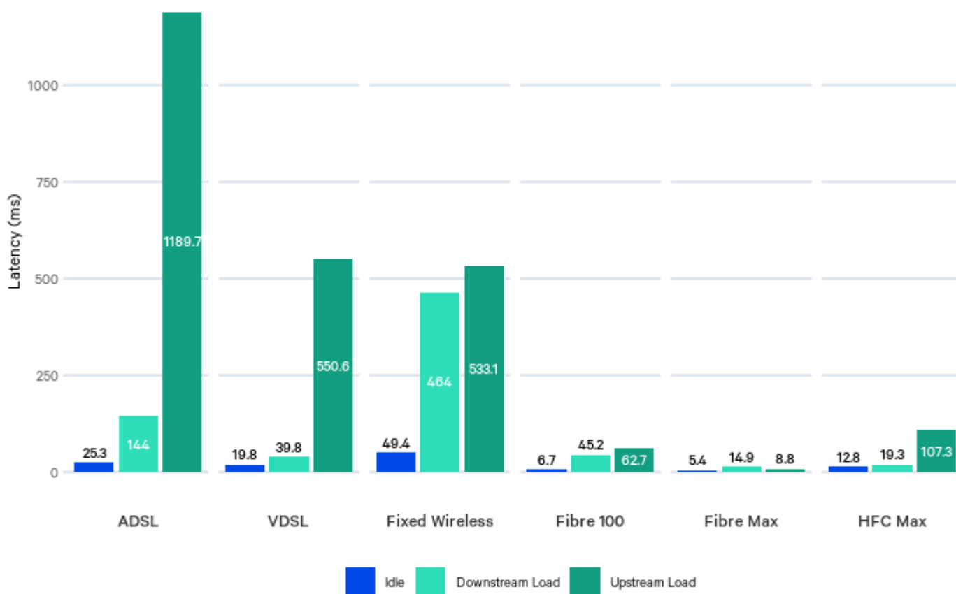
Figure 10 Average Latency Under Load to Test Servers by Plan. Lower is better.
