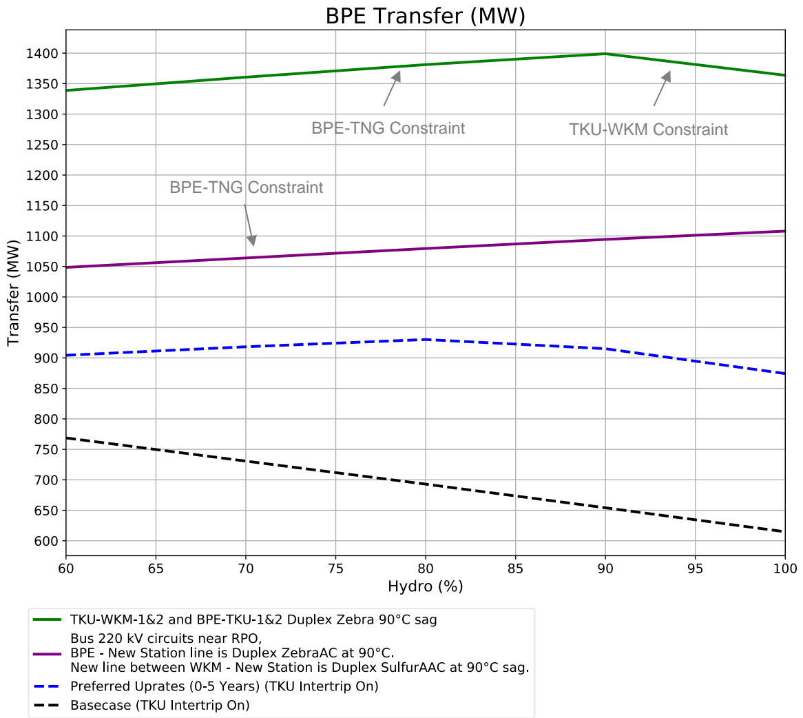
Figure 19: Option 14 transfer limits
