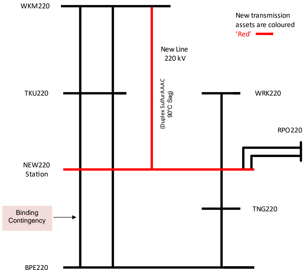
Figure 18: SLD for new station near RPO + duplex zebra reinforcement + new line, duplex Sulfur
