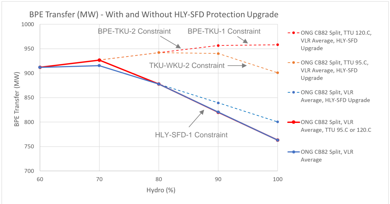
Figure 4: Bunnythorpe transfer limits with and without Huntly–Stratford 220 kV protection upgrade
