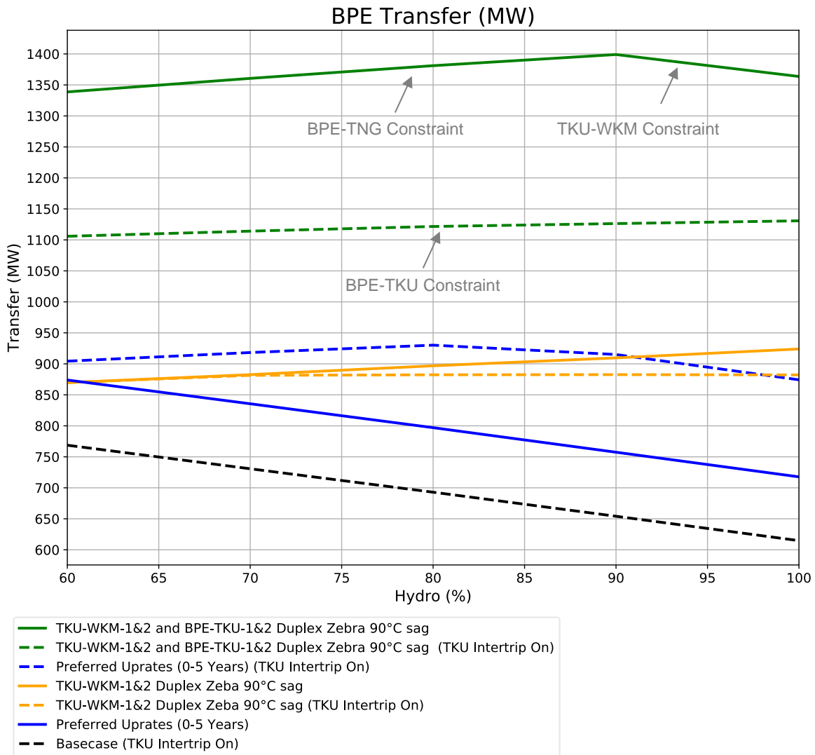
Figure 27: Three options with and without the TKU intertrip scheme in service
