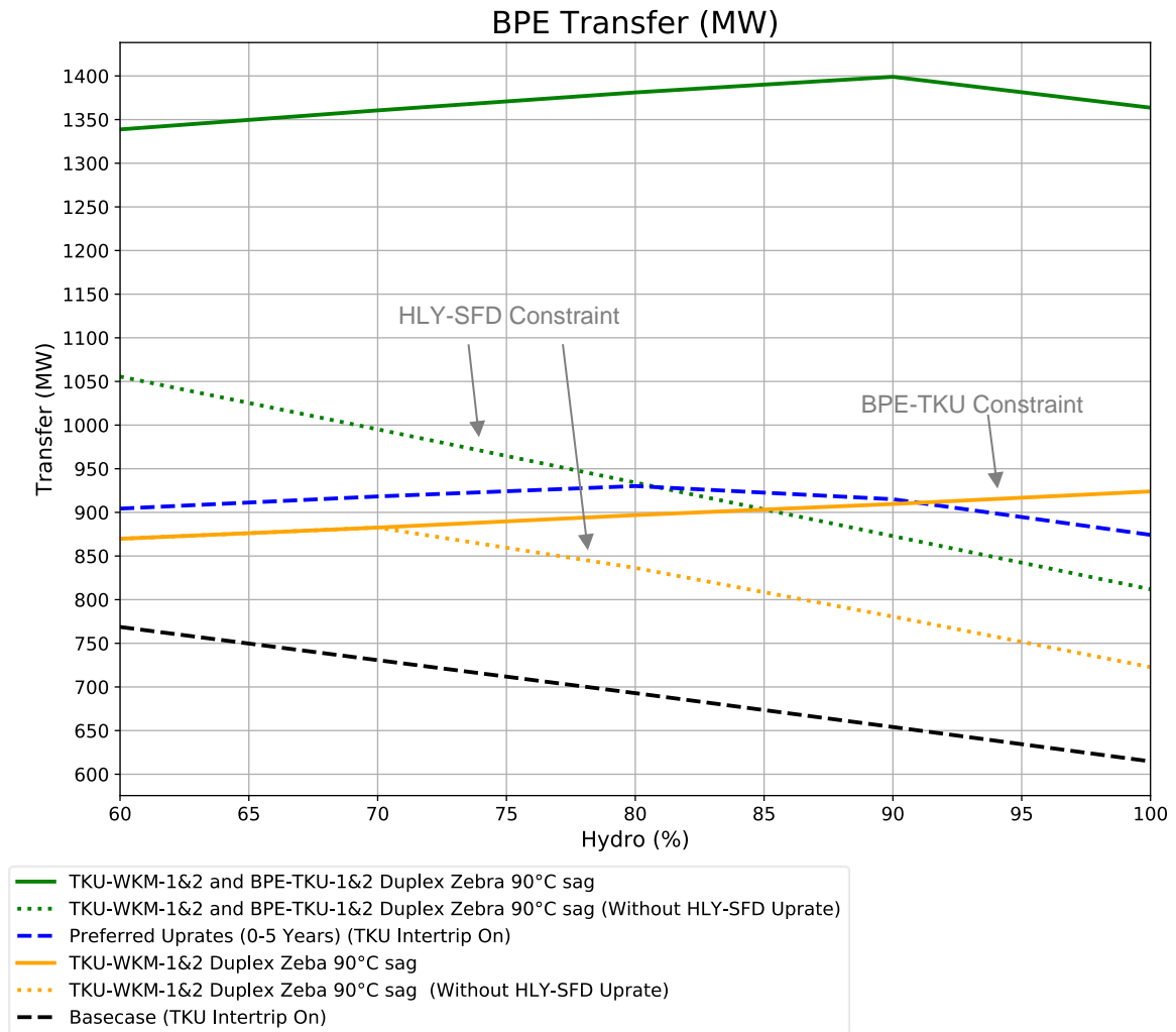
Figure 28: Transfer limit with and without the Huntly–Stratford protection upgrade
