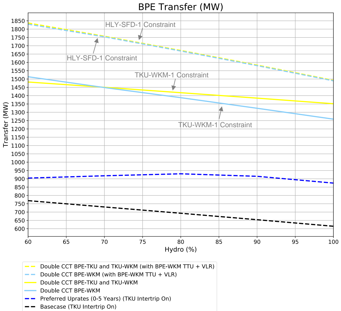
Figure 30: New 220 kV double circuit duplex line options between BPE and WKM with a 95°C TTU and VLR on the existing TKU-WKM and BPE-TKU 220 kV circuits
