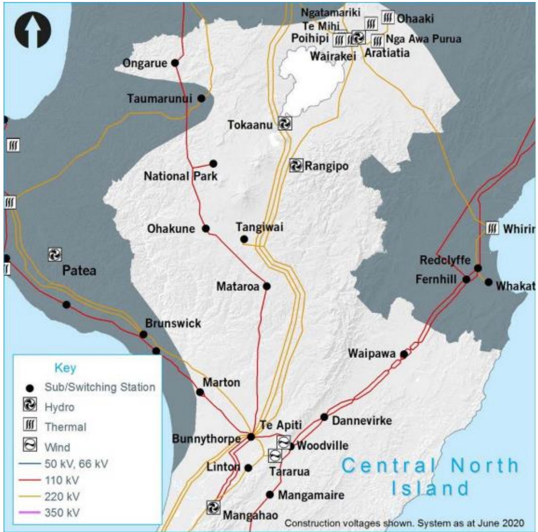
Figure 1: Geographic view of the Central North Island region transmission network
