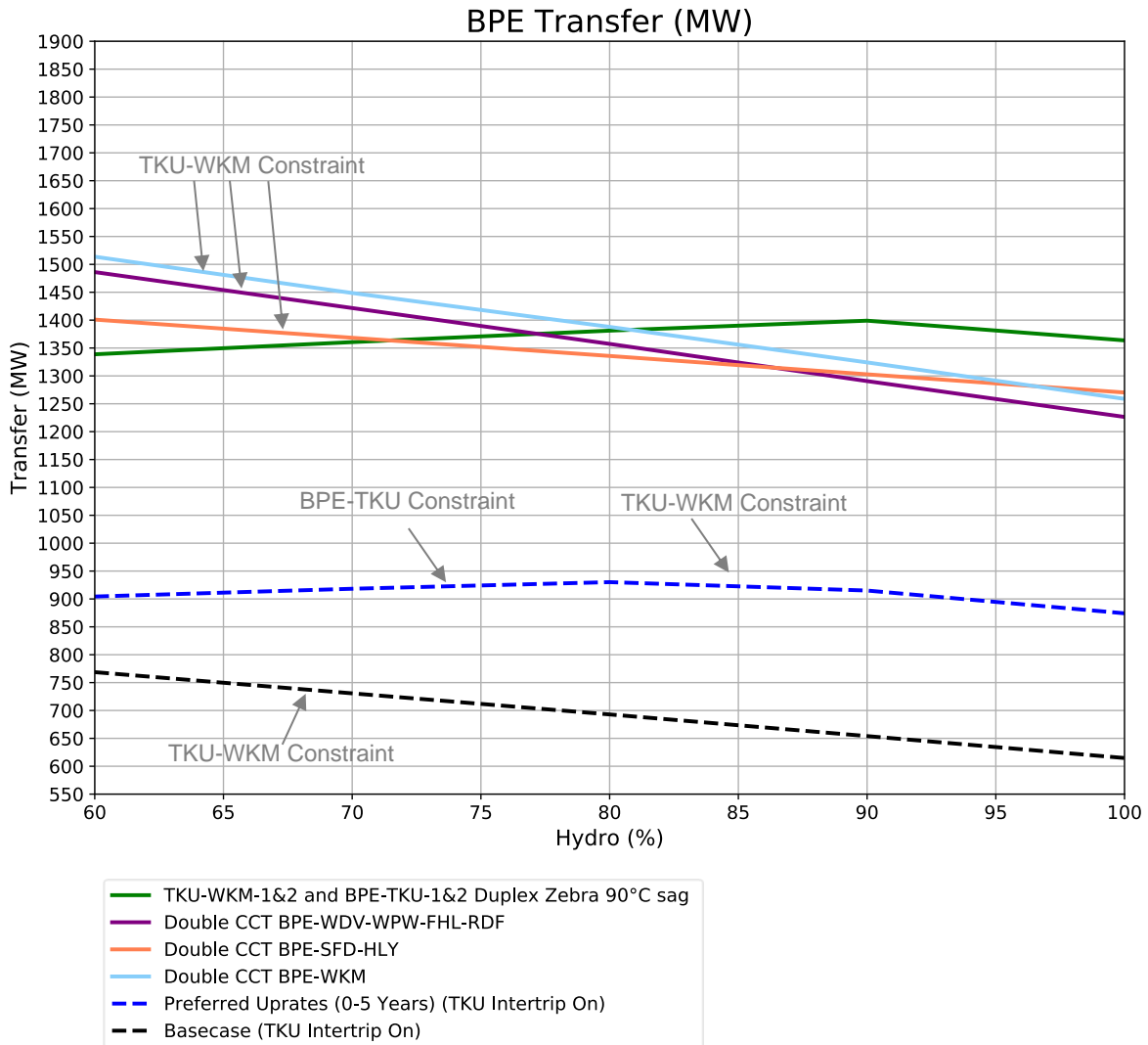
Figure 23: Option 17, 18 and 19 transfer limits
