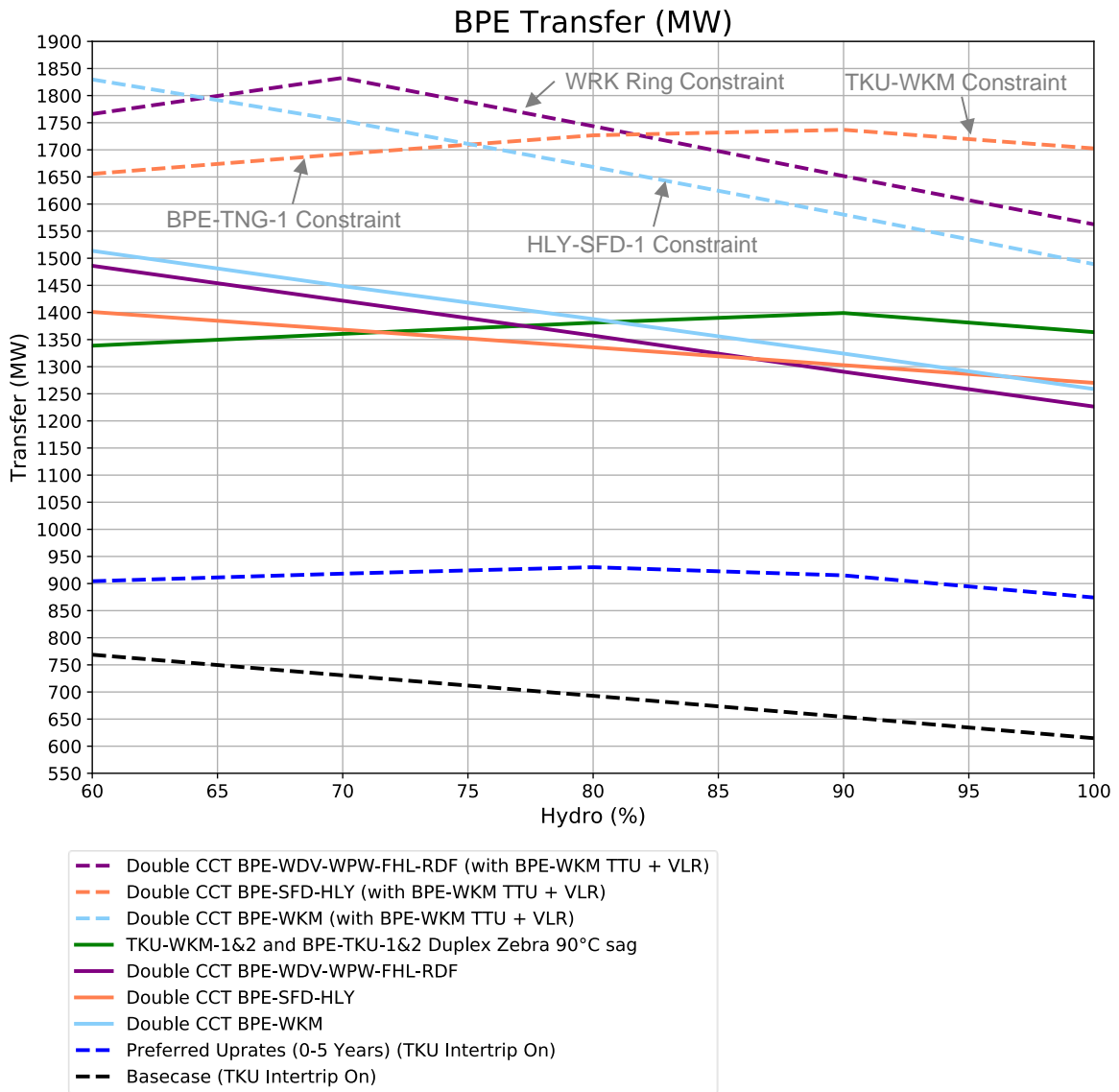
Figure 24: Option 17, 18 and 19 transfer limits with a 95°C TTU and VLR on the TKU-WKM and BPE-TKU 220 kV circuits
