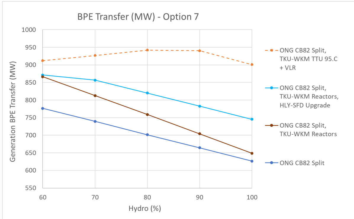
Figure 14: Bunnythorpe transfer limits with Option 7
