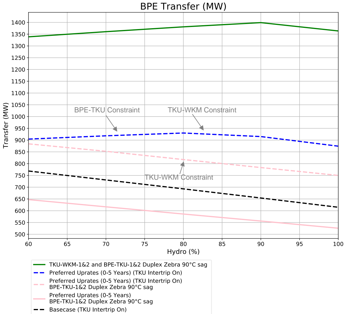
Figure 29: Duplexing post 95°C TTU on the Tokaanu–Whakamaru 220 kV circuits
