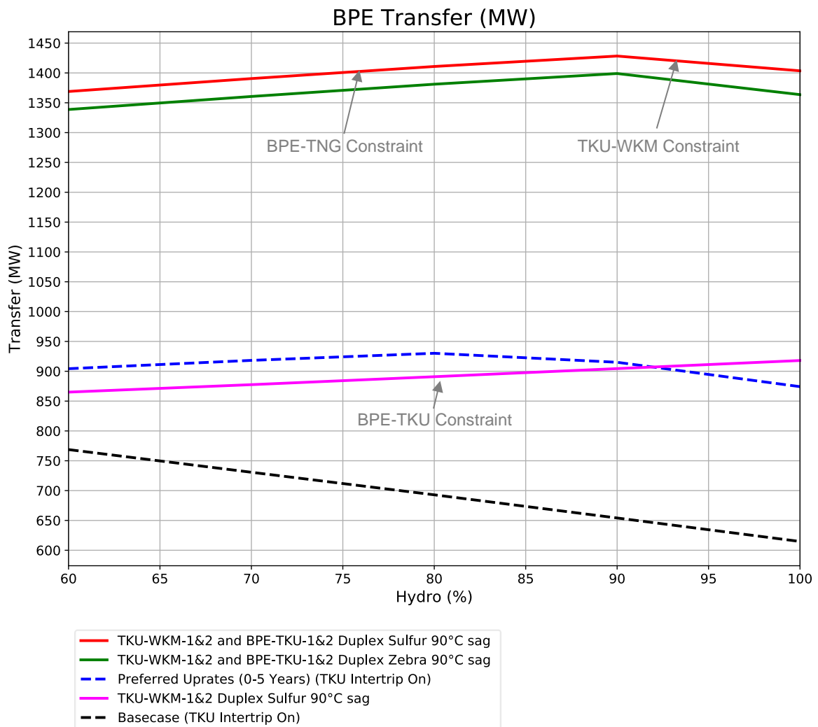
Figure 17: Option 12 and 13 transfer limits
