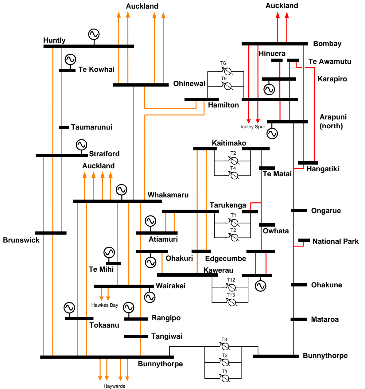
Figure 2: Single line diagram of the Central North Island transmission network
