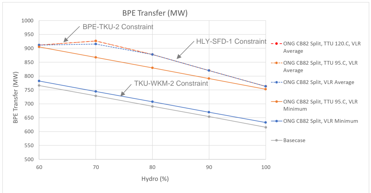
Figure 3: Bunnythorpe transfer limits for different Tokaanu–Whakamaru 220 kV TTU and VLR options
