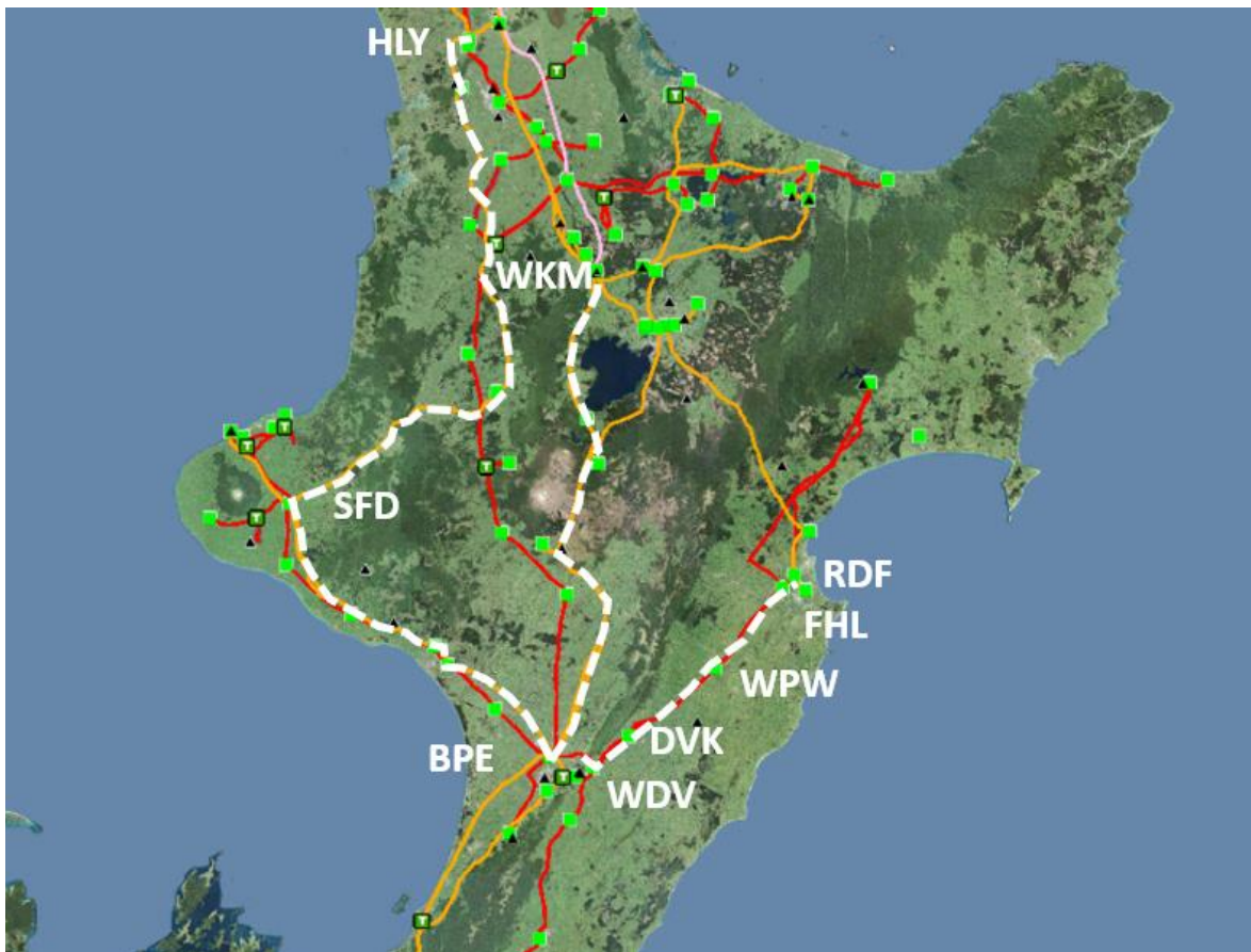
Figure 22: Geographical map of double circuit duplex options
