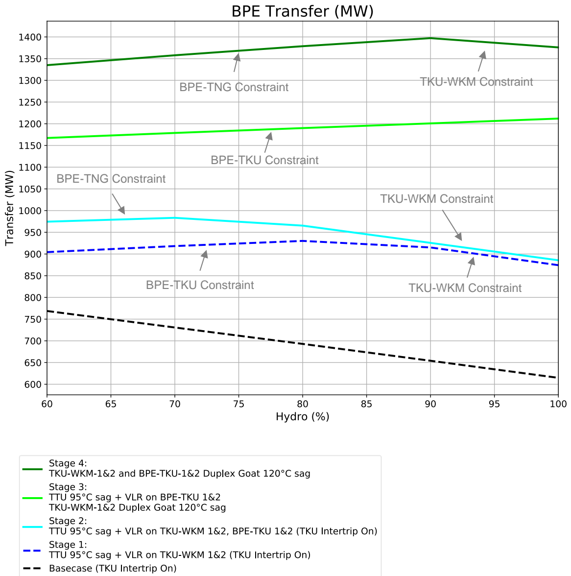
Figure 25: Thermal transfer increase for each stage of works on TKU–WKM 1&2 and BPE–TKU
