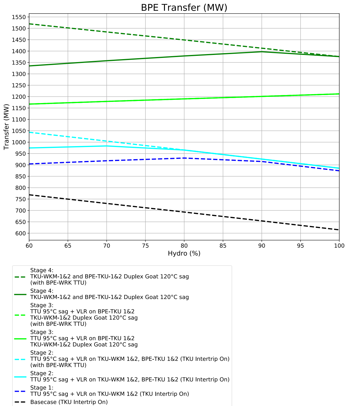
Figure 26: Thermal transfer increase for Stage 2 and Stage 4 with TTU on BPE–TNG, TNG–RPO, RPO–WRK
