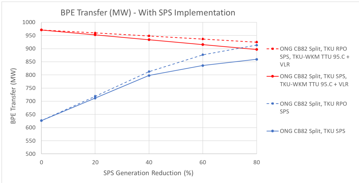
Figure 8: Bunnythorpe transfer limit with a SPS implemented at Tokaanu and Rangipo
