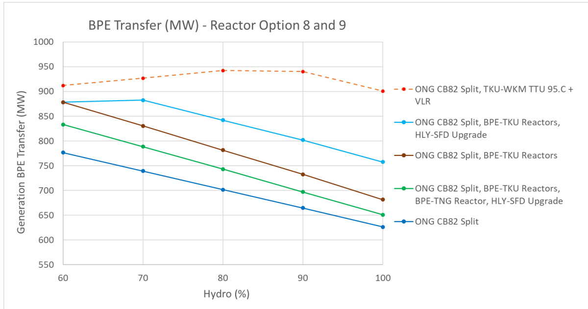
Figure 15: Bunnythorpe transfer limits with reactor Option 8 and 9
