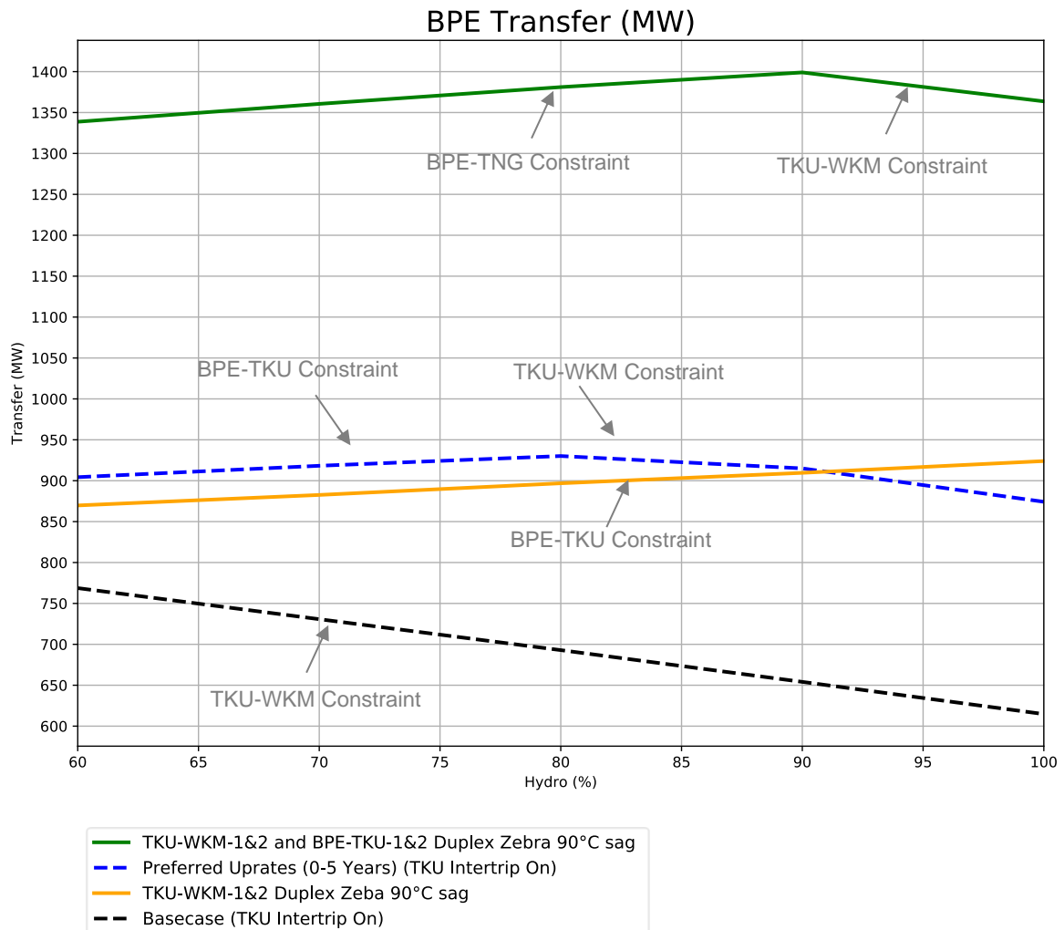
Figure 16: Option 10 and 11 transfer limits
