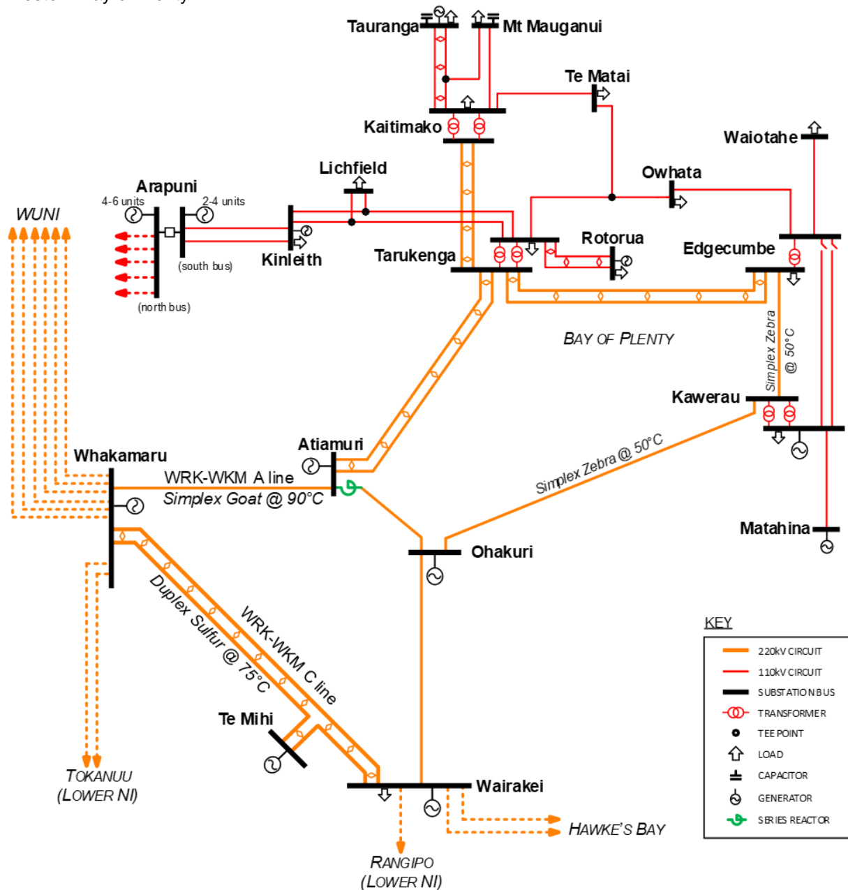
Figure 3: transmission schematic of the Wairakei Ring and the Bay of Plenty regional grid (with Atiamuri series reactor and the Edgecumbe – Kawerau 110kV system split implemented)
