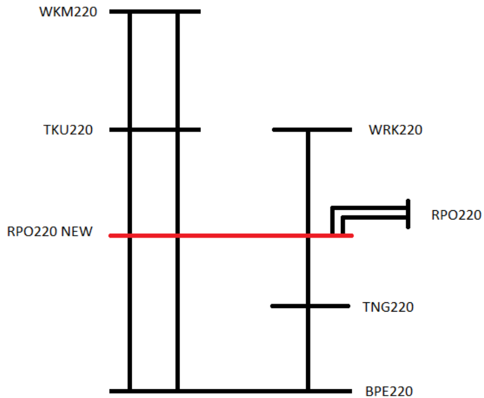
Figure 12: Option 6 schematic
