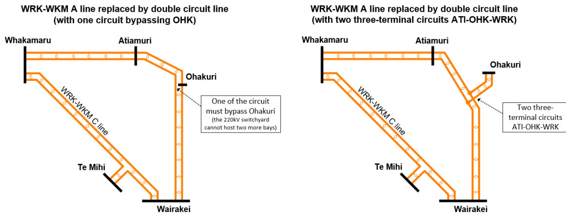
Figure 13: simplified transmission schematic of the options for the WRK–WKM A line replacement
