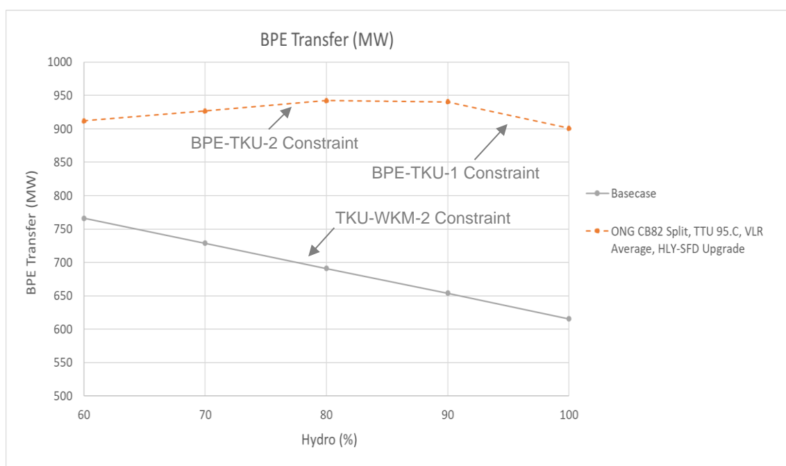
Figure 7: Bunnythorpe transfer limits, base case compared against the TKU-WKM TTU 95°C + VLR option
