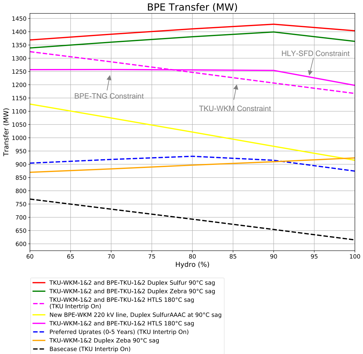
Figure 21: Option 16 transfer limits
