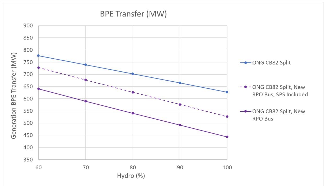
Figure 13: Bunnythorpe transfer limit with new Rangipo 220 kV bus
