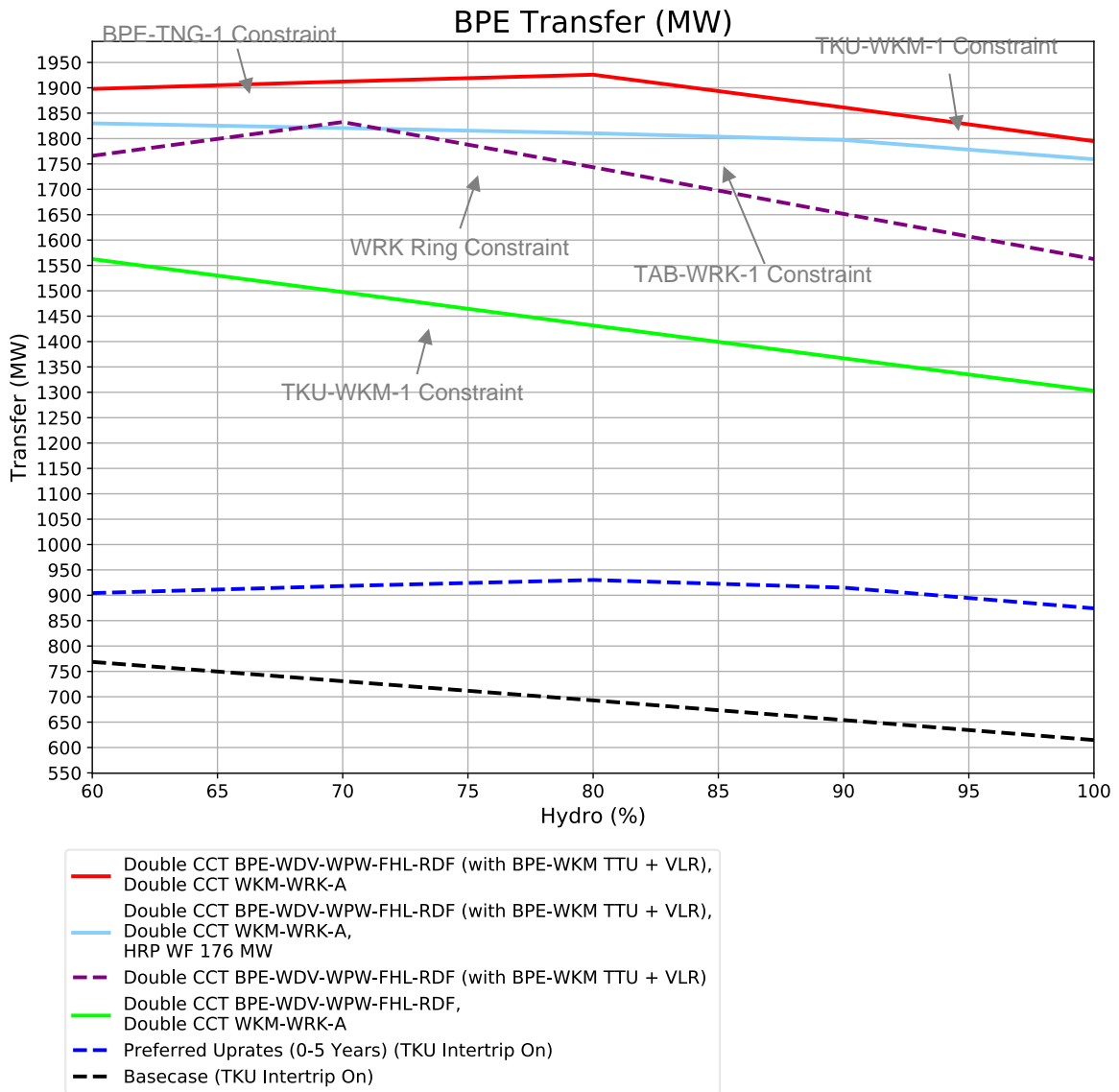
Figure 31: Wairakei Ring sensitivity study, Option 18 + new double circuit WKM-WRK-A Line
