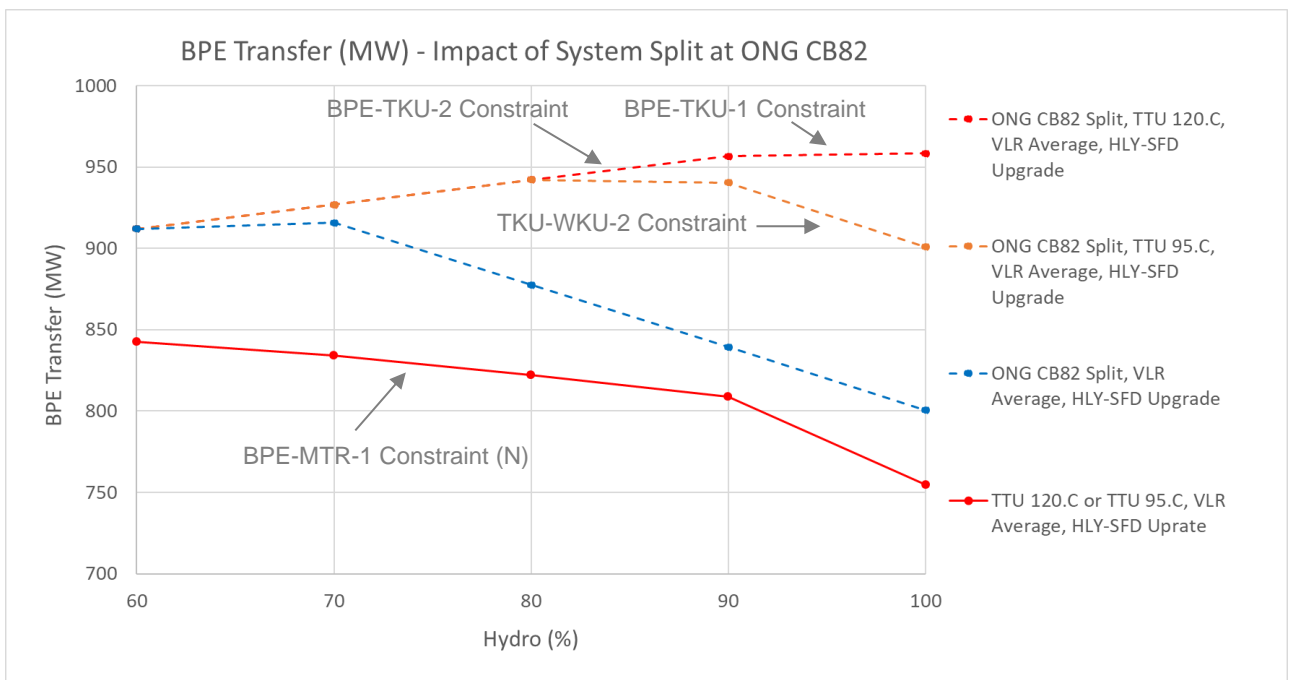
Figure 5: Bunnythorpe transfer limits with and without a split at Ongarue CB82
