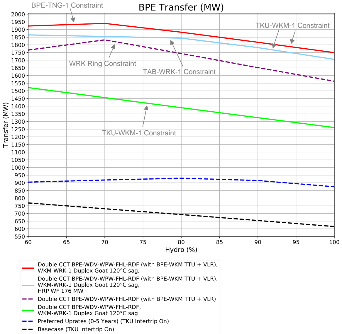
Figure 32: Wairakei Ring sensitivity study, Option 18 + duplex existing WKM-WRK 220 kV circuit
