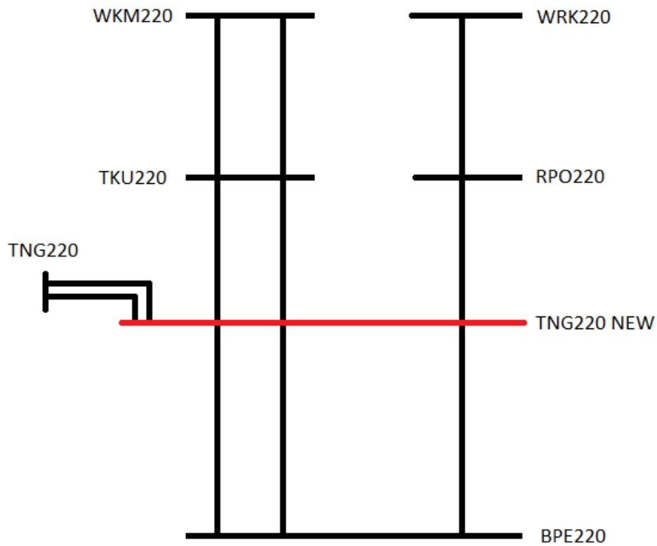
Figure 10: Option 5 schematic
