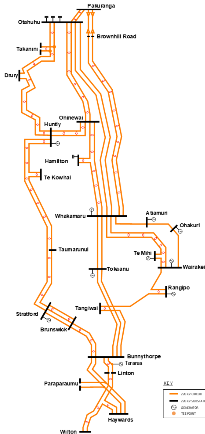
Figure 2: Simplified North Island grid backbone schematic
