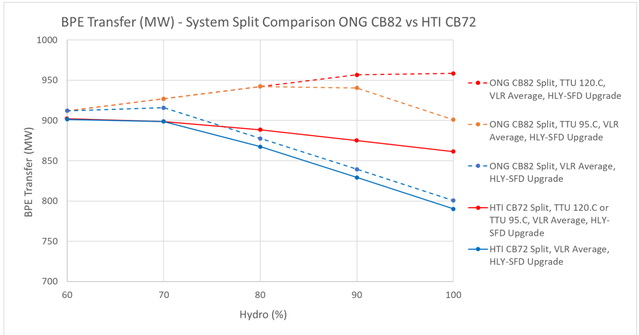
Figure 6: Bunnythorpe transfer limits with a split at Ongarue CB82 versus a split at Hangatiki CB72
