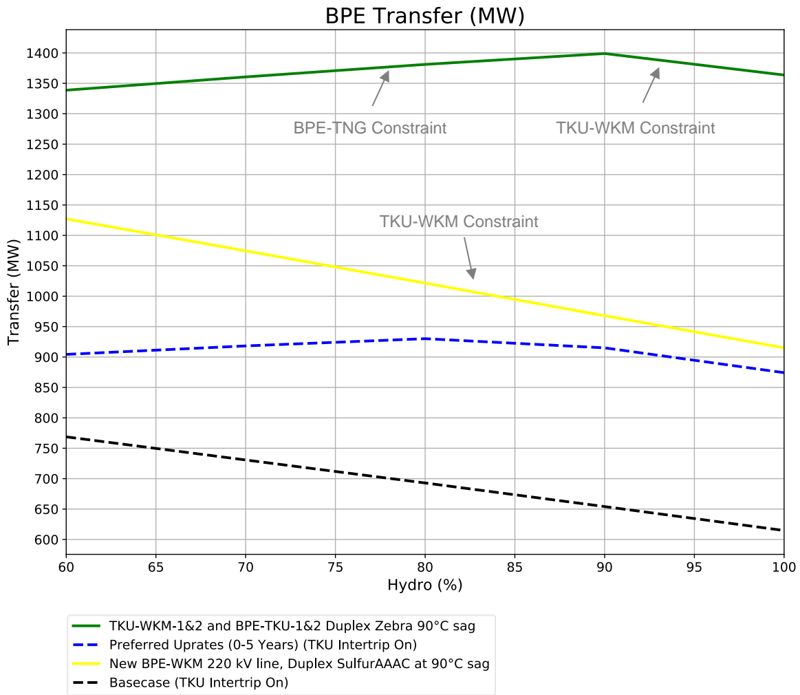
Figure 20: Option 15 transfer limits
