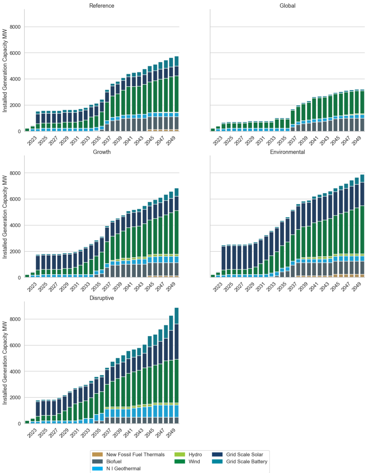
Figure 10: New installed generation capacity for each scenario
