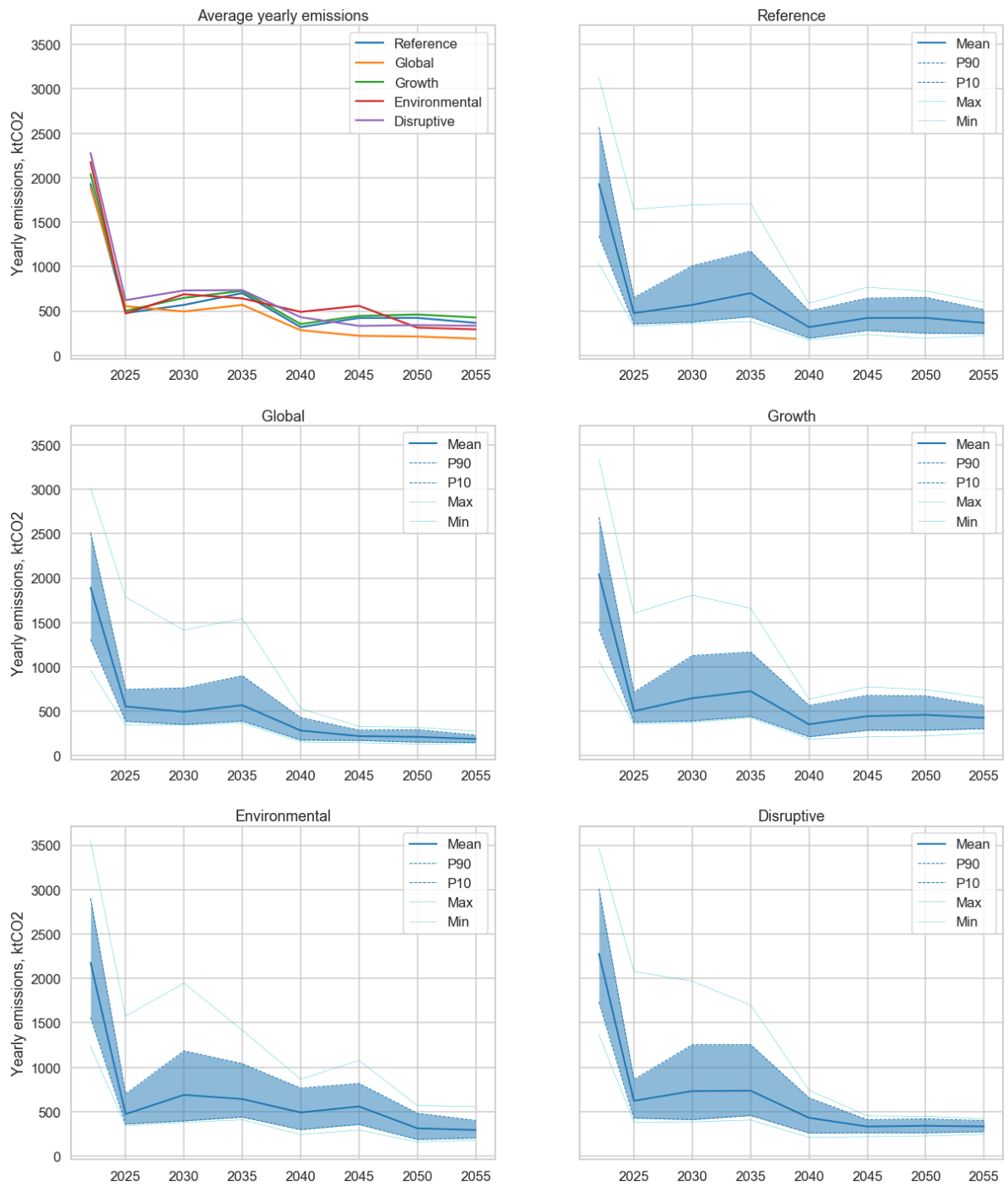
Figure 29: Yearly greenhouse gas emissions, preferred option with Tiwai leaves in 2024 and HVDC fourth cable in 2027
