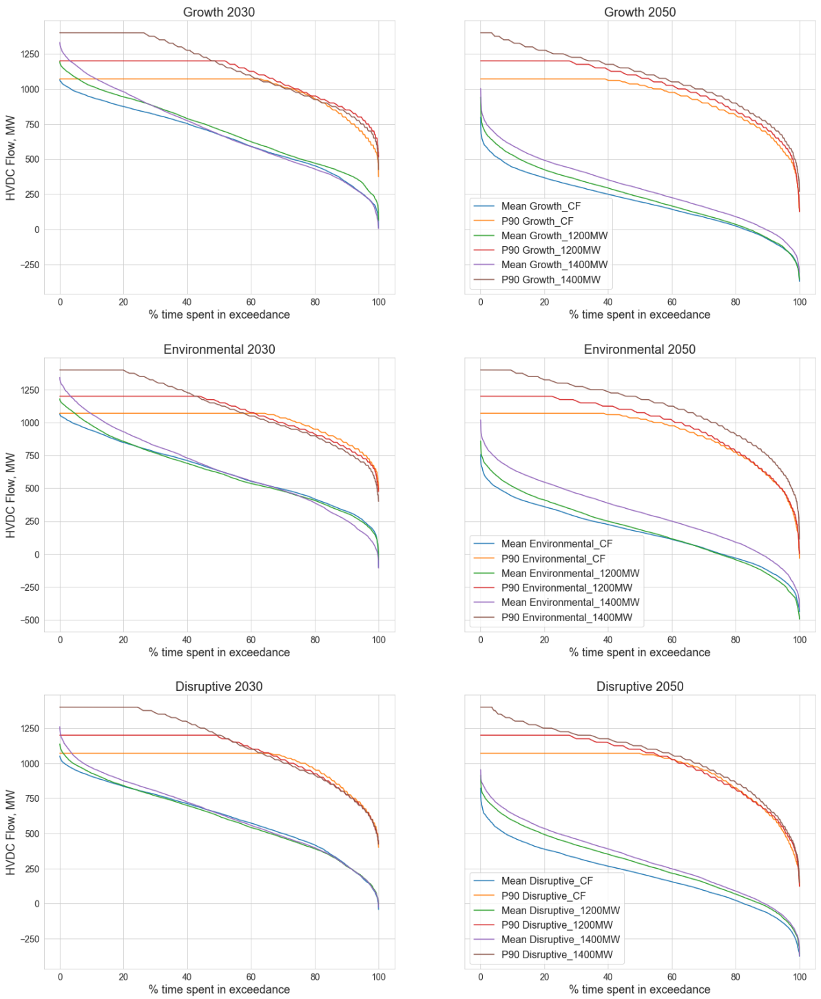
Figure 20: HVDC flows for the preferred option
